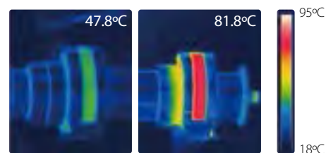
Temperature comparison at the same overrunning speed
